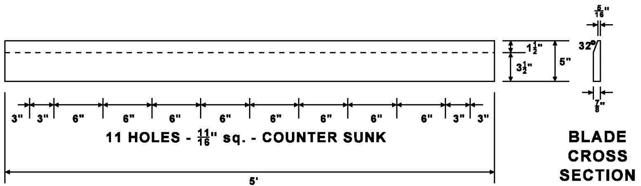
FIVE FOOT BLADE SECTION
