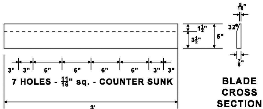
THREE FOOT BLADE SECTION
